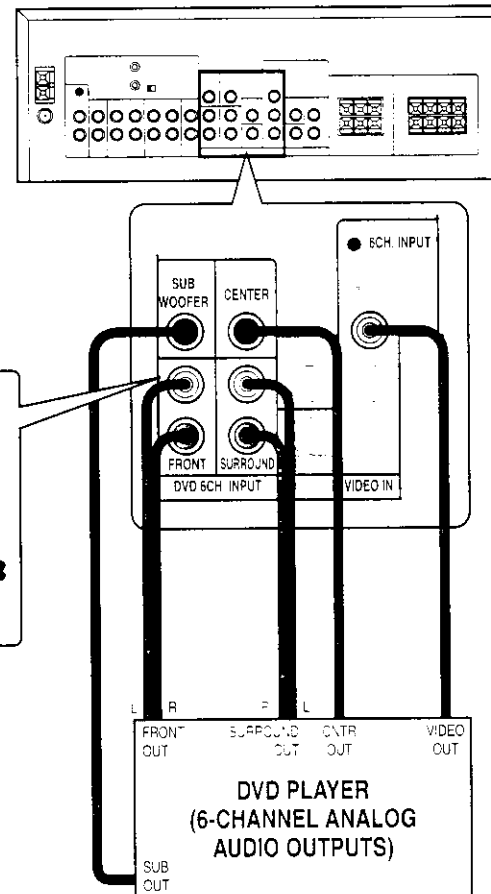
VR-205 RECEIVER
